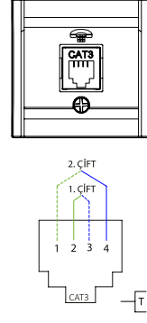
Numeris Telephone Socket Outlet (RJ11 CAT3) Nümeris Priz (RJ11 CAT3) XXX-XXXXXX-221
