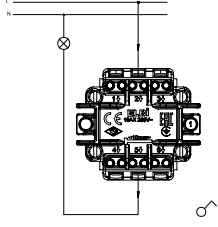
Control Switch Light Light Anahtar XXX-XXXXXX-205
