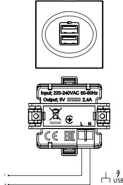
Double USB Charger 5V 2,1A USB Sarj Prizi 5V 2,1A Çiftli XXX-XXXXXX-143
