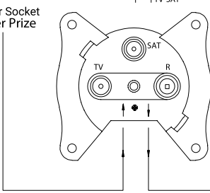
Shielded TV Socket Outlet End Of Line TV Prizi Ekranlı - Sonlu XXX-XXXXXX-273
