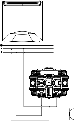
Socket Outlet Earthed Child Protection With Hinged Lid Çocuk Korumalı Kapaklı Topraklı Priz XXX-XXXXXX-219
