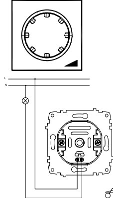
Dimmer Illuminated (1000W) Işıklı Dimmer (1000W) XXX-XXXXXX-192
