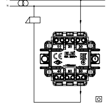
12V Illuminated Labelled Control Switch Bell 12V Işıklı İsimli Zil Anahtar XXX-XXXXXX-208
