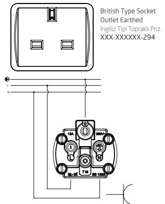
Flush Mounted 3G Earthed Socket Outlet Sıva Altı Üçlü Topraklı Priz XXX-XXXXXX-819
