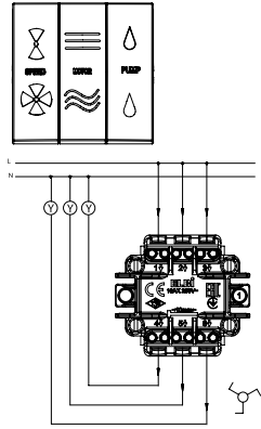
3Gang 1Way Hvac Switch 3'lü Klima Anahtarı XXX-XXXXXX-279
