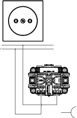
Socket Outlet Without Earthed Priz XXX-XXXXXX-215
