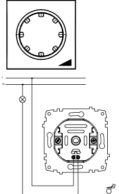
RC Led Dimmer (5-300W) RC Led Dimmer (5-300W) XXX-XXXXXX-310
