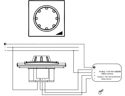
Dimmer 1-10V Dimmer 1-10V XXX-XXXXXX-316
