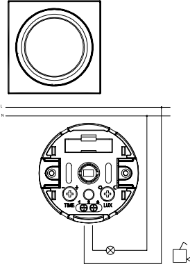
Relay Motion Sensor Röleli Hareket Sensörü XXX-XXXXXX-262
