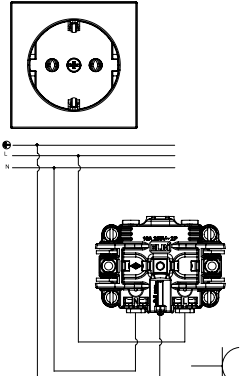
Socket Outlet Earthed Topraklı Priz XXX-XXXXXX-217
