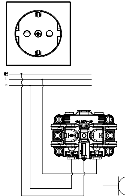
Socket Outlet Earthed Child Protection Çocuk Korumalı Topraklı Priz XXX-XXXXXX-243
