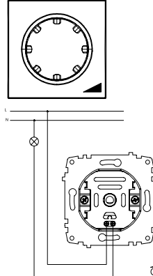
RC Led Dimmer (5-60W) RC Led Dimmer (5-60W) XXX-XXXXXX-308
