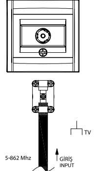
TV Socket Outlet End Of Line TV Priz - Sonlu XXX-XXXXXX-246
