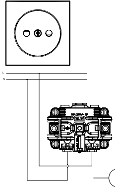
Child Protection Socket Without Earthed Çocuk Korumalı Priz XXX-XXXXXX-286
