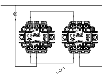
1Gang 2Way Switch Intermediate Ara Veavien (Permutatör) XXX-XXXXXX-214
