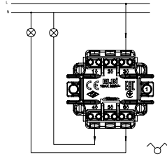
Control Switch Bell Zil Anahtar XXX-XXXXXX-207
