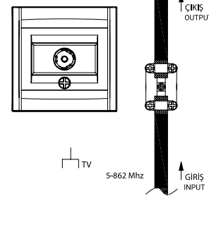
TV Socket Outlet Through Line TV Priz - Geçişli XXX-XXXXXX-224
