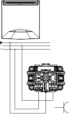
Socket Outlet Earthed With Hinged Lid Kapaklı Topraklı Priz XXX-XXXXXX-218
