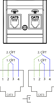
Double Numeris Telephone Socket Outlet (2 x RJ11 CAT3) İkili Nümeris Priz (2 x RJ11 CAT3) XXX-XXXXXX-222
