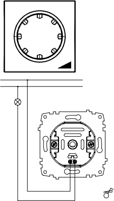
Dimmer 500W CE Dimmer 500W CE XXX-XXXXXX-144
