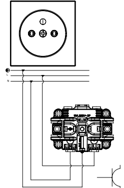
UPS Socket Outlet With Earthed Pin UPS Priz XXX-XXXXXX-268
