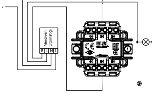
1Gang 2Way Illuminated Switch Işıklı Veavien XXX-XXXXXX-210
