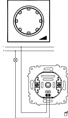
Dimmer (1000W) Dimmer (1000W) XXX-XXXXXX-112
