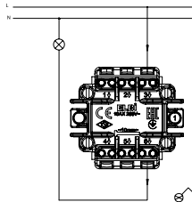
Control Switch Illuminated Light Işıklı Light Anahtar XXX-XXXXXX-206
