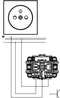
Child Protection UPS Socket Outlet Earthed Pin Çocuk Korumalı UPS Priz XXX-XXXXXX-263
